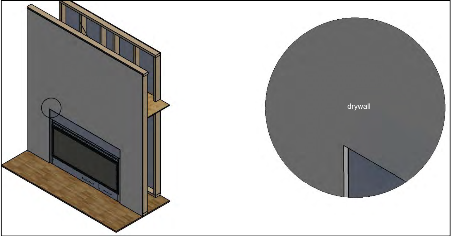
Figure 10.0.01: Drywall to Fireplace (not flush)
