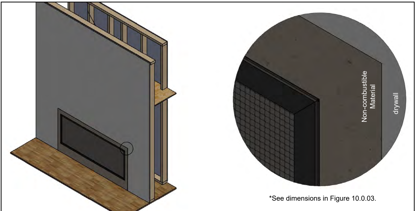
Figure 10.0.02: Drywall to Fireplace (not flush)
