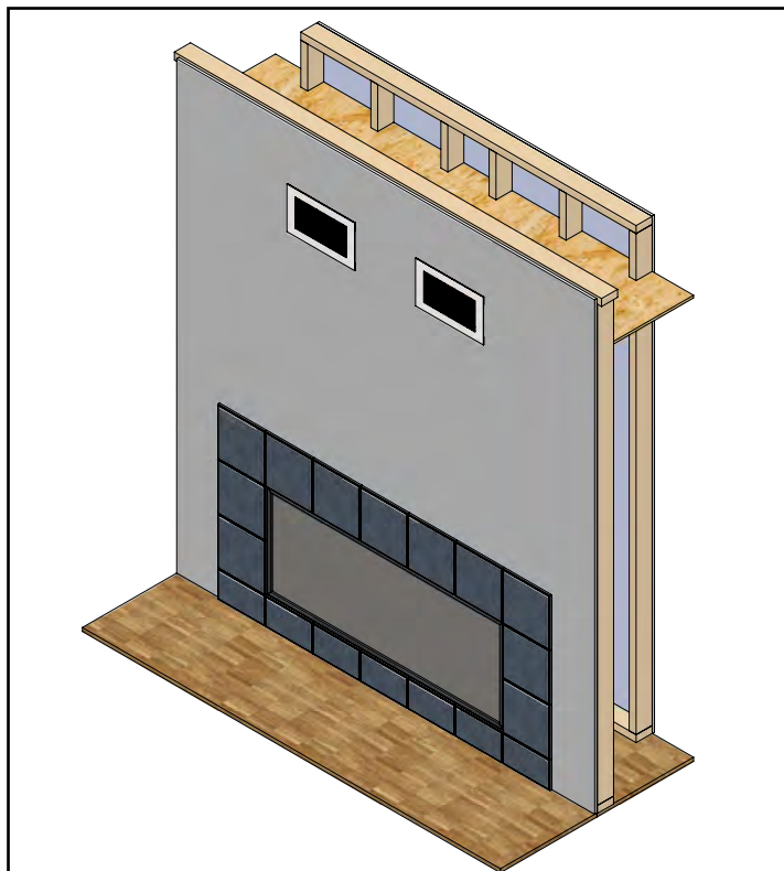
Figure 7.2.04: I.H.E.A.T. with dual 12" discharge heads (999-IHT-51212)
