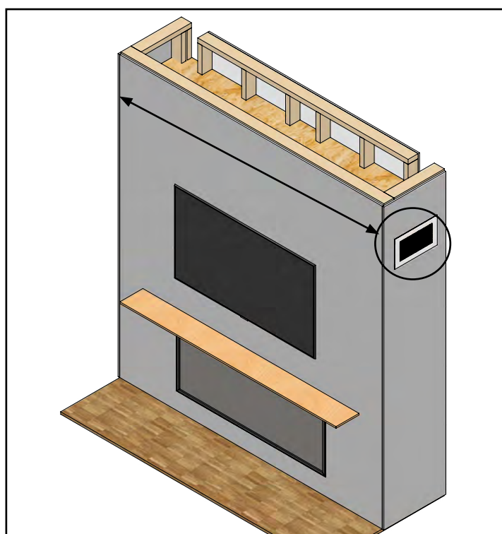
Figure 7.2.06: I.H.E.A.T. with television and dual 12" discharge heads (999-IHT-51212) - shown with non-combustible finishing material
