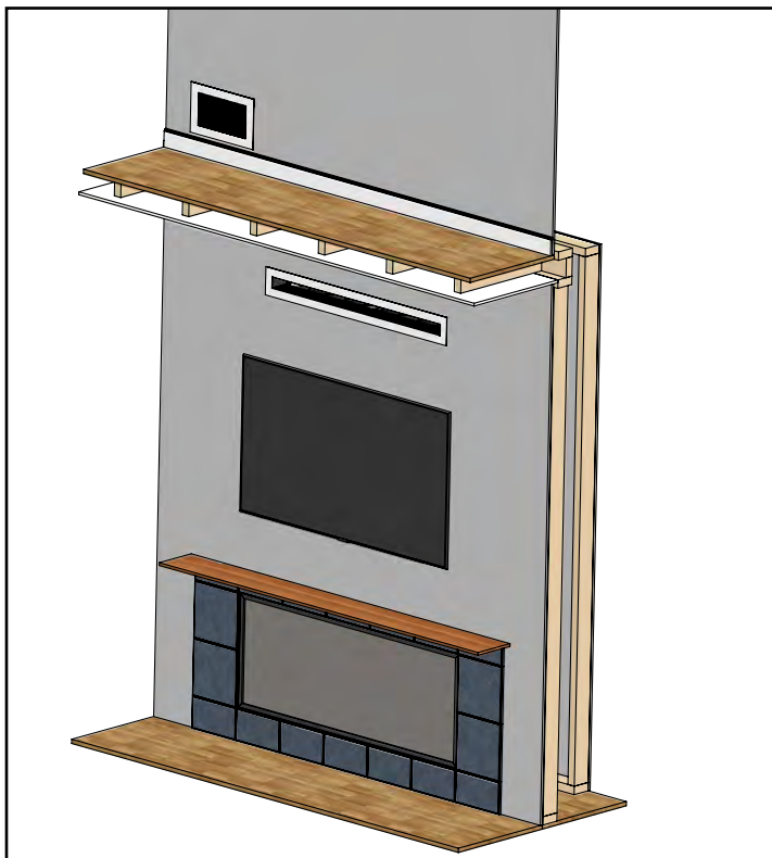
Figure 7.2.03: I.H.E.A.T. second storey heat distribution with television (999-IHT-54012)
