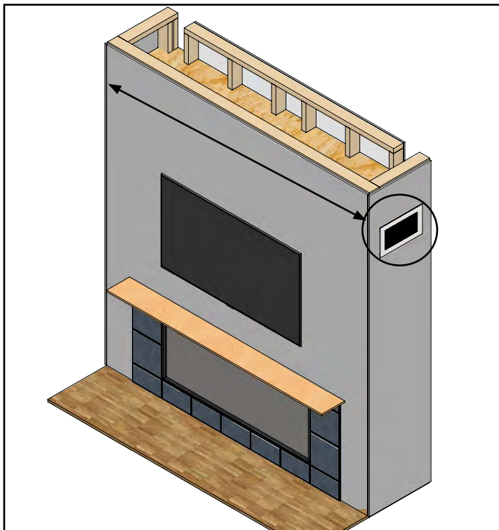
Figure 7.2.05: I.H.E.A.T. with television and dual 12" discharge heads (999-IHT-51212) - shown with non-combustible tile
