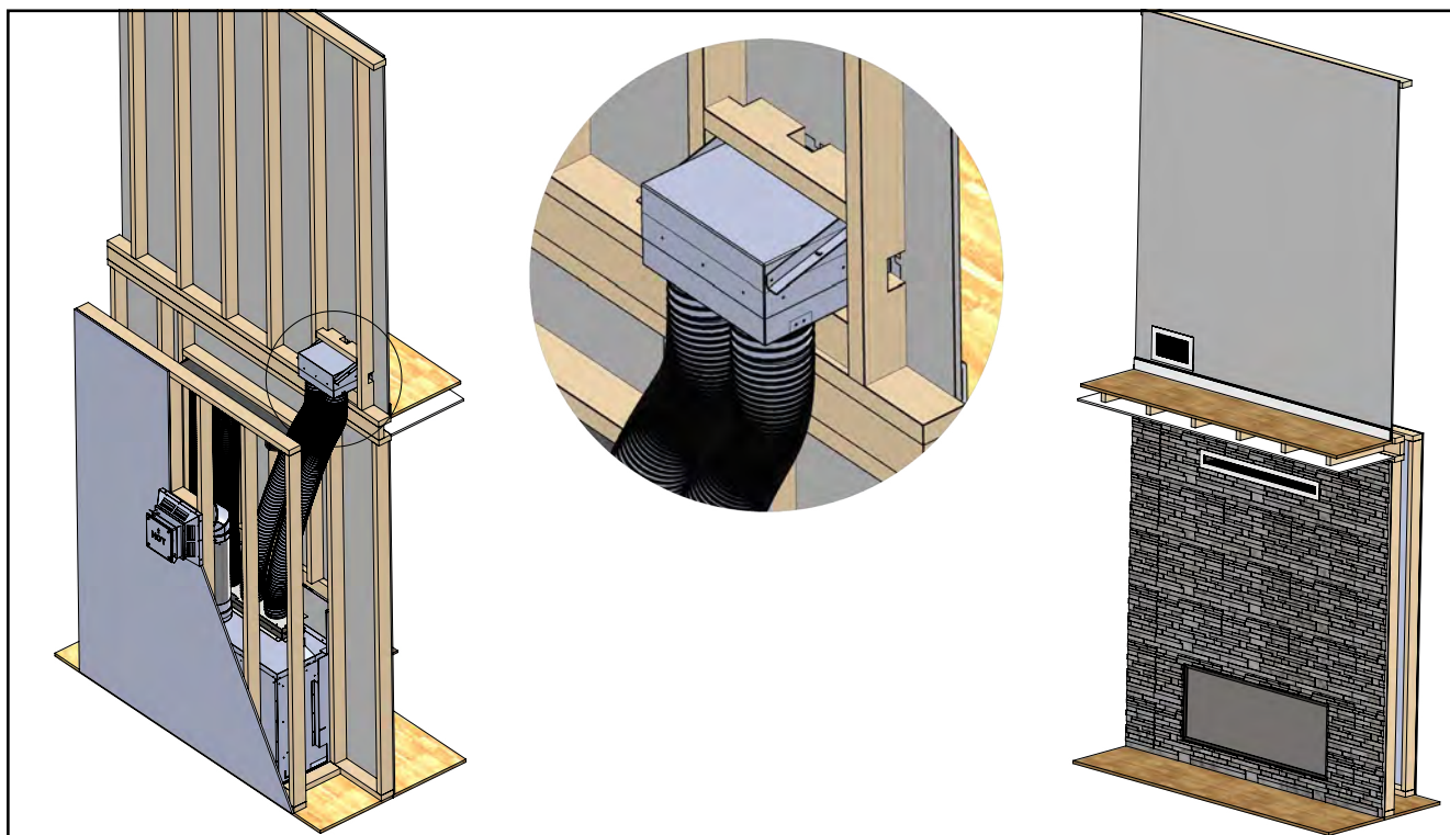
Figure 7.2.02: I.H.E.A.T. second story heat distribution (999-IHT-54012)
