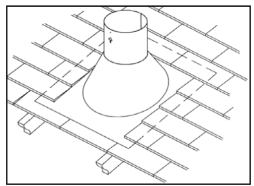
Figure 10.005: Flashing Installation
